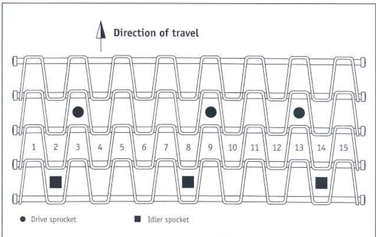
TYPICAL SPROCKET SETUP
